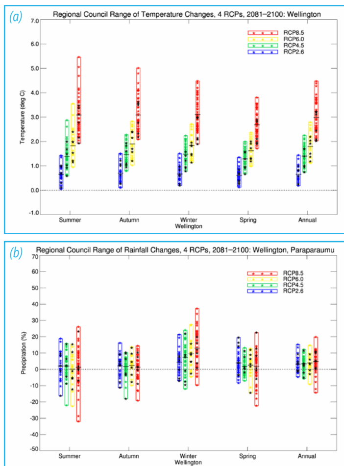
Range of model outcomes for temperature (a) and rainfall (b) for 2090
