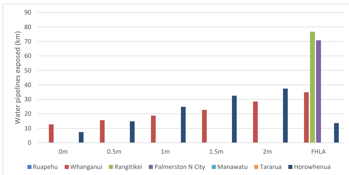
Figure 6-14: Length of water pipelines in territorial areas exposed to a 1:100-year storm tide event at present day and future levels of SLR, as well as in the flood hazard area.
