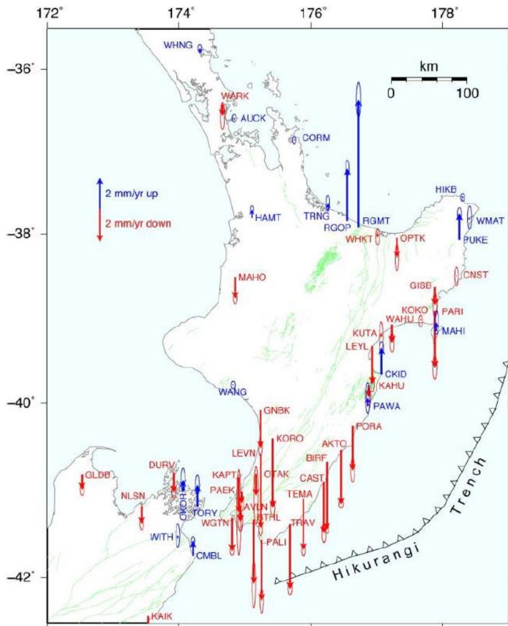
Figure 10-7: Average vertical land movements (mm/yr) for near-coastal continuous GPS sites across central New Zealand regions. Source: Beavan and Litchfield (2012).
