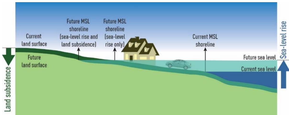
Figure 10-2: Difference in mean sea level (MSL) shoreline between absolute and local (relative) SLR where land subsidence occurs.
