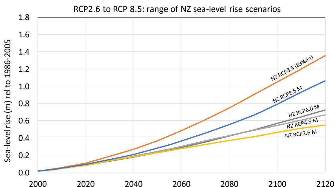
Figure 10-9: SLR scenarios for New Zealand seas, based on a set of median projections for all four RCPs (based on Church et al., 2013b) plus a higher 83rd percentile RCP8.5 projection (based on (Kopp et al., 2014)). The M next to the RCP on the plot stands for median. Note: for New Zealand seas, SLR projections will be around 5-10% higher than the global mean SLR published by IPCC, so between 2.5 to 5 cm by 2100 has been added to the median global average projections, and 7.5 cm to the higher scenario.
