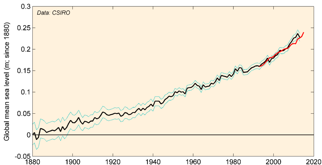
Figure 10-3: Cumulative changes in global mean sea level (MSL) since 1880, based on a reconstruction of long-term tide gauge measurements to end of 2013 (black) and recent satellite measurements to end 2015 (red). Lighter lines are the upper and lower bounds of the likely range ( \pm 1 standard deviation) of the MSL from available tide gauges, which is a function of the number of measurements collected and the precision of the methods. Tide gauge data from Church and White (2011), updated to 2013; satellite data from CSIRO (2016).
