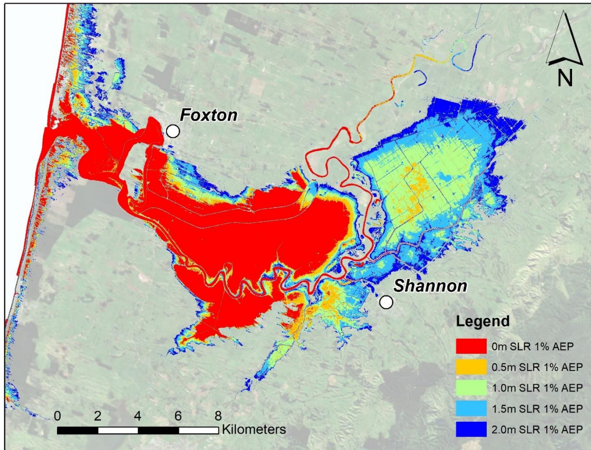
Figure 6-2: 1% AEP storm tide + sea-level rise elevations exposure in the Foxton area. Source: Paulik et al. (2019b).
