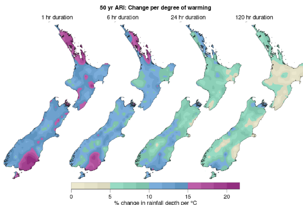
Figure 10-1: Change in the 50-year rainfall event magnitude for four different event durations. Each map combines all 24 different RCM simulations and shows the percentage change per degree of warming. Source: Ministry for the Environment (2018a).
