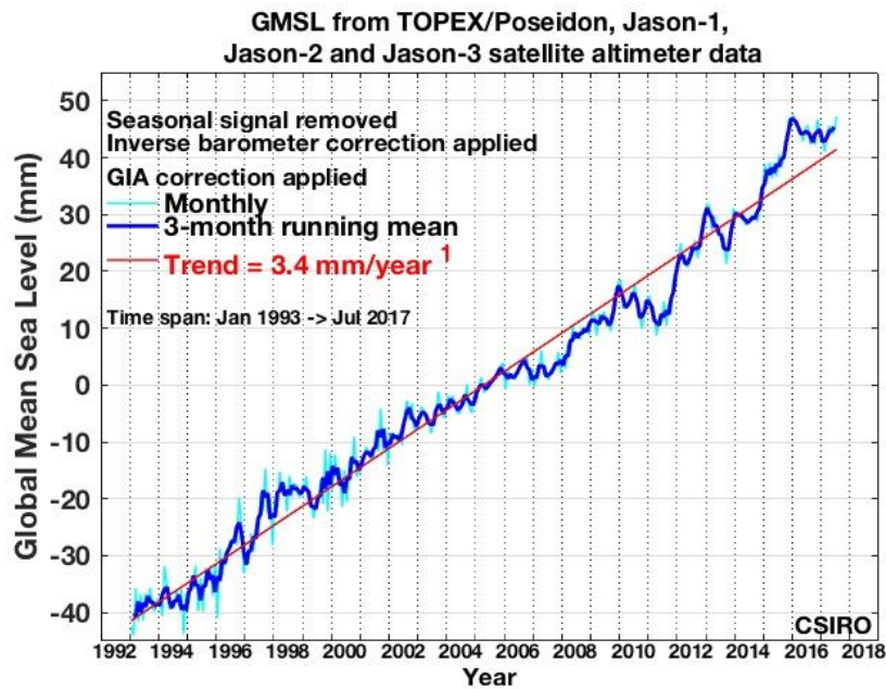
Figure 10-4: Time series and trend in global average sea level over the satellite era from January 1993 to July 2017. Adjustments for glacial isostatic adjustment (GIA), following crustal response to the last Ice Age, and inverted barometer (annual air pressure differences) have been made. Retrieved from CSIRO web site: http://www.cmar.csiro.au/sealevel/sl_hist_last_decades.html
